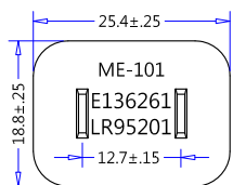
ME-101 (1-15P, Non-Polarized) (Dimensions of Plug Face)
