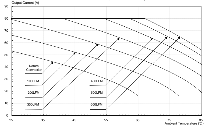
Figure 34: Output current vs. ambient temperature and air velocity @ Vin=12V, Vout=3.3V (Worst Orientation)
