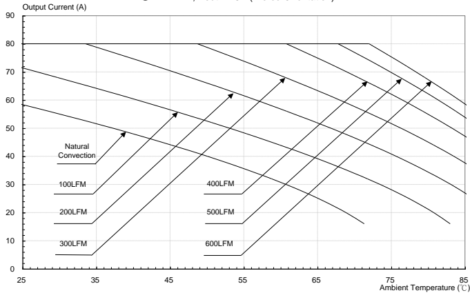
Figure 33: Output current vs. ambient temperature and air velocity @ Vin=12V, Vout=2.5V (Worst Orientation)
