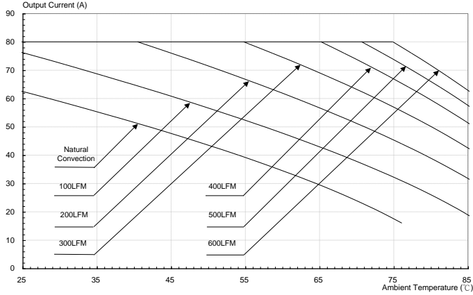
Figure 32: Output current vs. ambient temperature and air velocity @ Vin=12V, Vout=1.8V (Worst Orientation)
