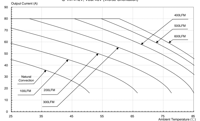
Figure 35: Output current vs. ambient temperature and air velocity @ Vin=12V, Vout=5.0V (Worst Orientation)
